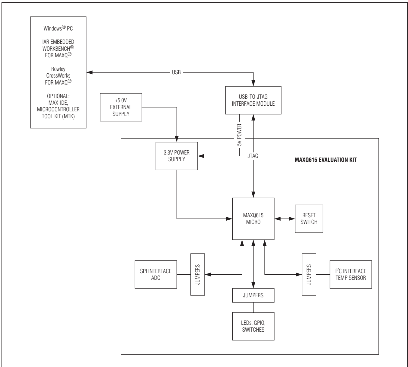
Figure 2. MAXQ615 EV Kit System Block Diagram
