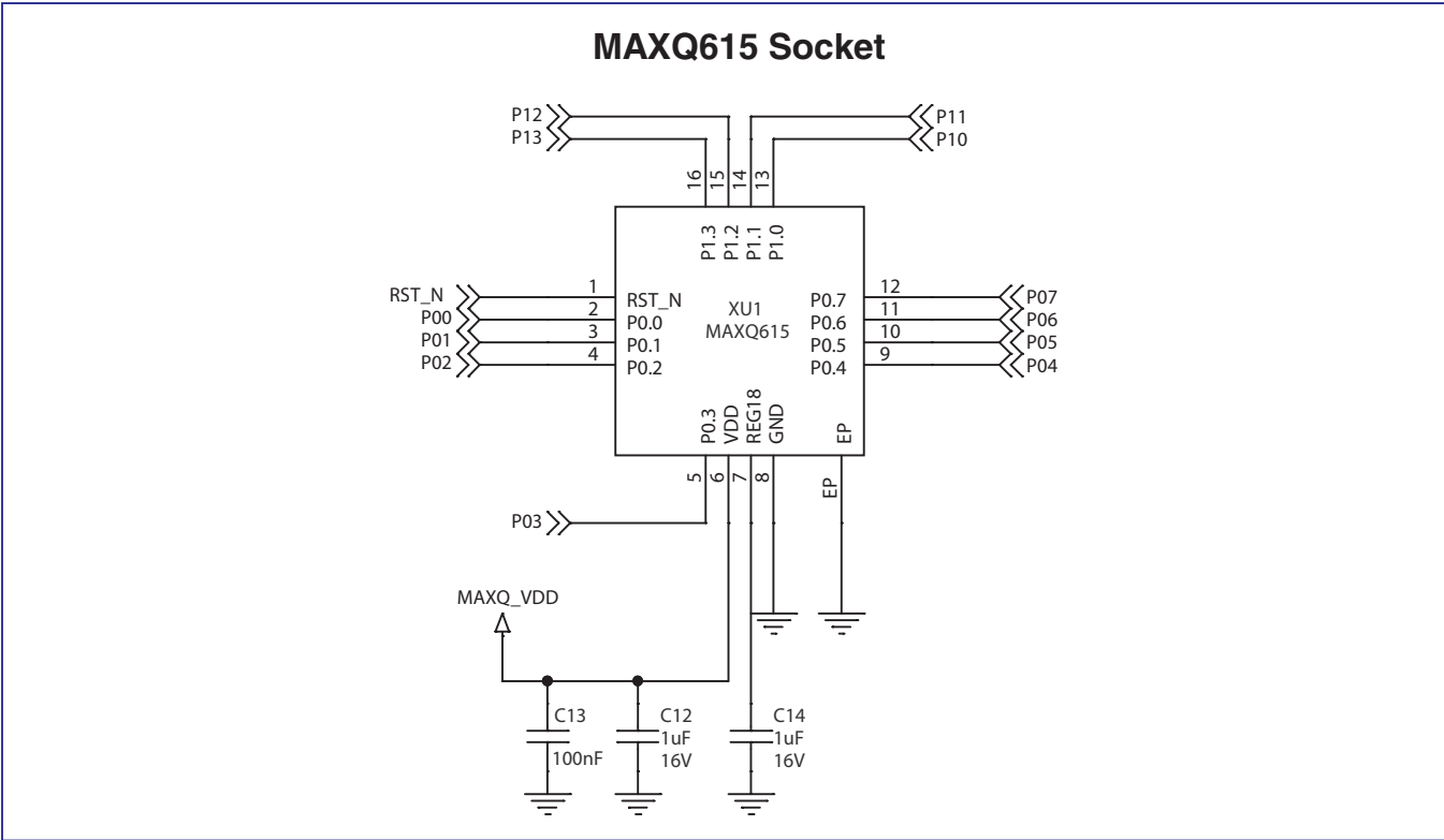
Figure 4. MAXQ615 EV Kit Schematics (Sheet 2 of 2)
